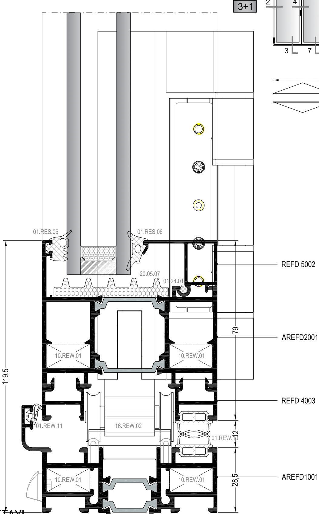
KATLANIR KAPI İÇE AÇILIM DETAYI FOLDING DOOR INWARD OPENING DETAIL
