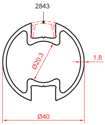
2842 0.822 kg/m
